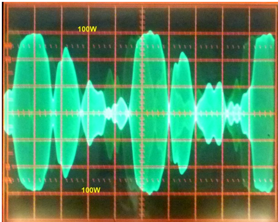
Figure 4: SSB RF envelope at 100W PEP. Note ALC compression on voice peaks.
