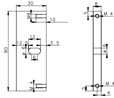
Plaque support de la caméra Audine
